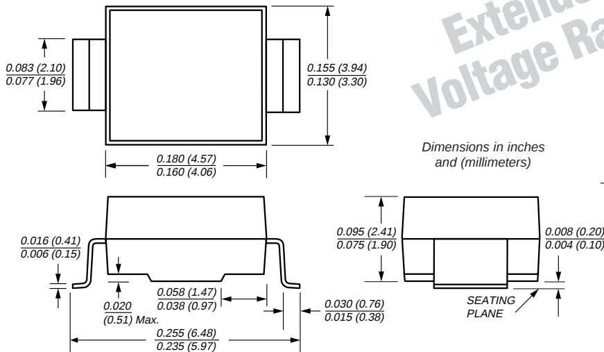
DO-215AA (SMBG)
