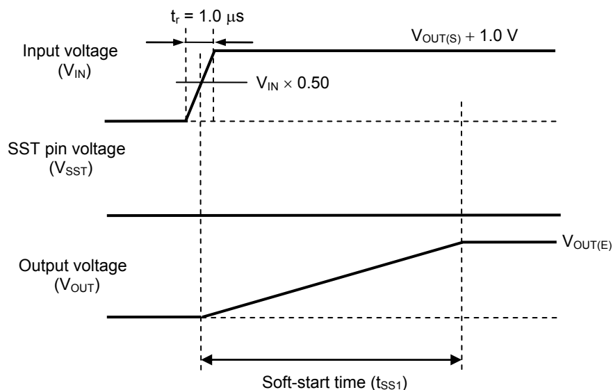
Figure 34 V_{SST} = \text{"L"}
