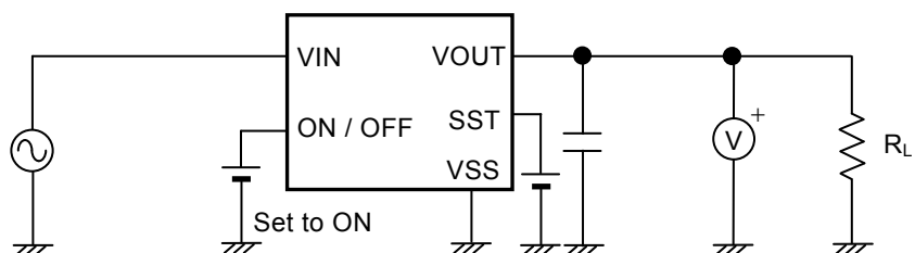
Figure 23 Test Circuit 10
