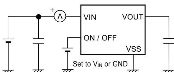
Figure 15 Test Circuit 2
