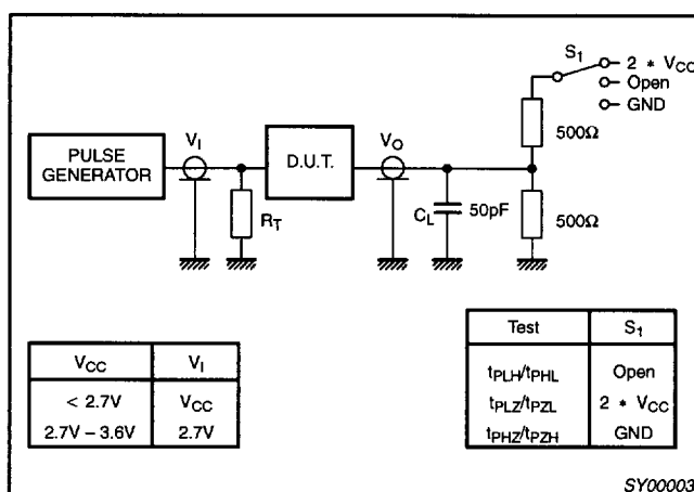
Waveform 4. Load circuitry for switching times.
