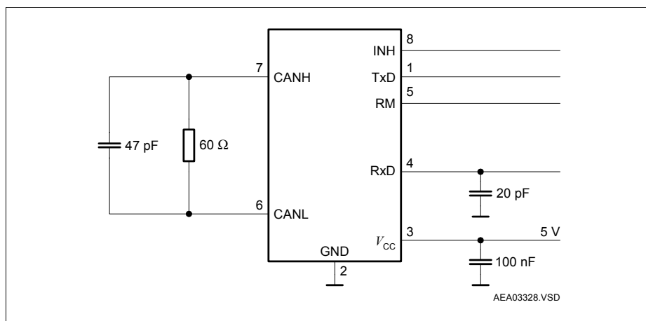
Figure 7 Test Circuit for Dynamic Characteristics (5 V Version)
