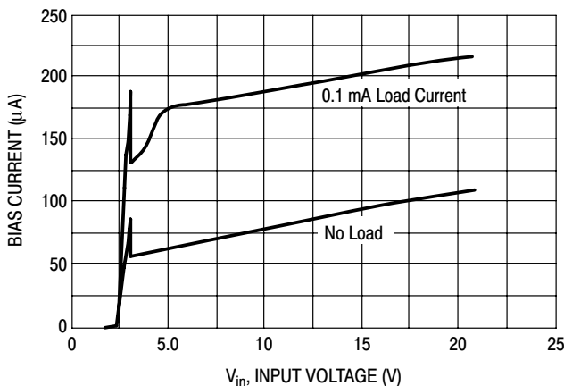
Figure 4. Input Current
