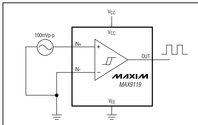
Figure 5. Zero-Crossing Detector
