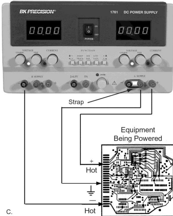
Fig. 8. Series Tracking Operation Grounding Possibilities
