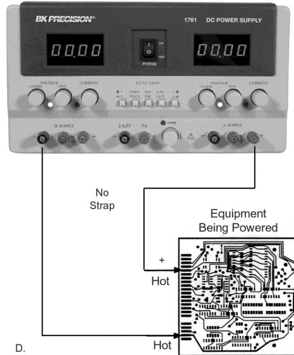
Fig. 8. Series Tracking Operation Grounding Possibilities
