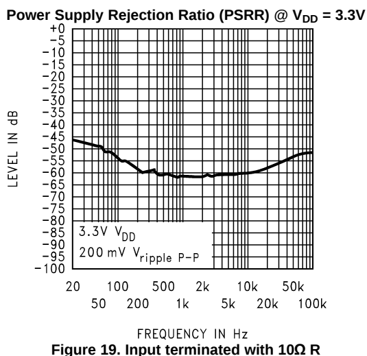
Figure 19. Input terminated with 10\Omega R
