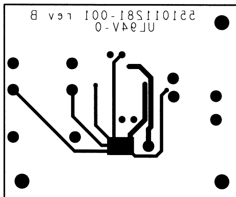
Figure 39. Bottom Layer
