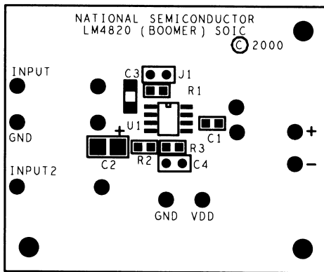
Figure 37. Silk Screen
