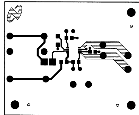
Figure 41. Top Layer
