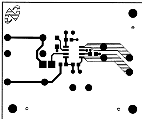
Figure 38. Top Layer
