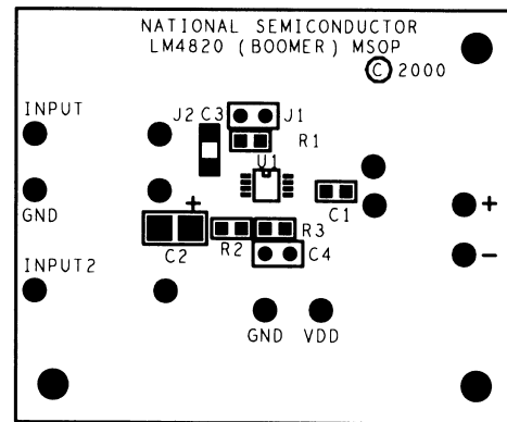
Figure 40. Silk Screen
