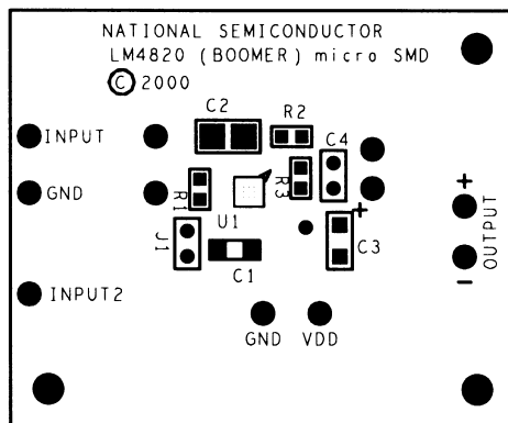
Figure 31. Silk Screen
