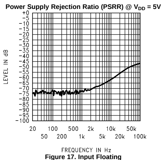
Figure 17. Input Floating
