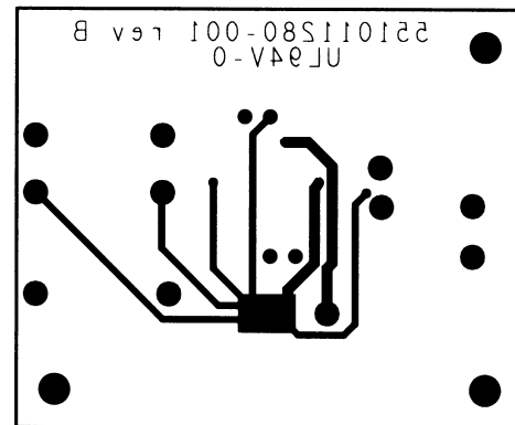
Figure 42. Bottom Layer
