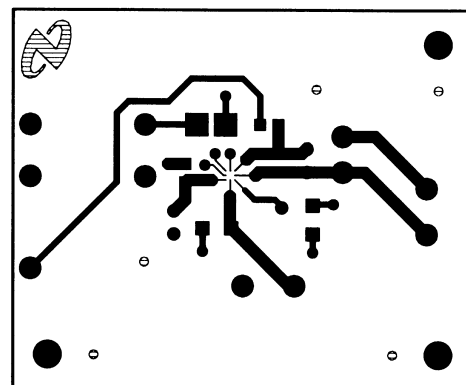
Figure 32. Top Layer
