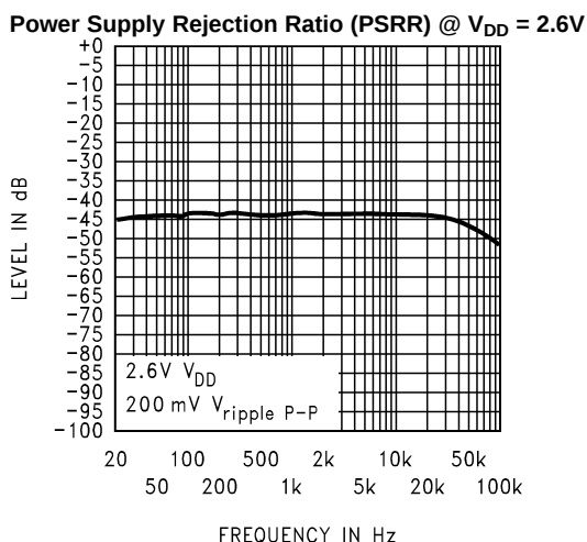
Figure 18. Input terminated with 10\Omega R
