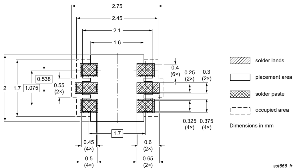
Fig. 31. Reflow soldering footprint for SOT666
