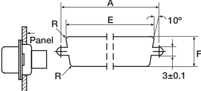
Front Panel Mounting
