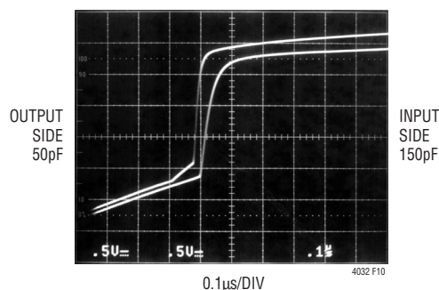
Input-Output Connection t_{PIH}
