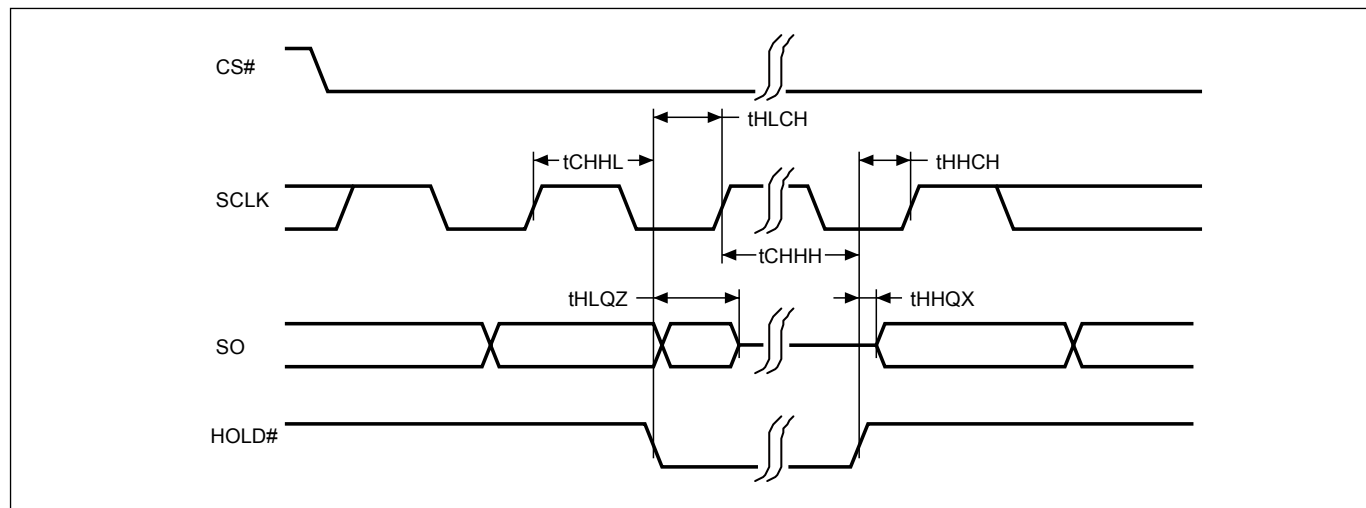
Figure 4. Hold Timing
