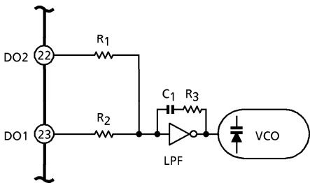
When using LPF in common (filter constants switched over by placing DO in high-impedance state)
