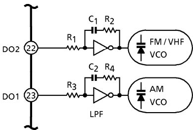
When setting time constant in each band
