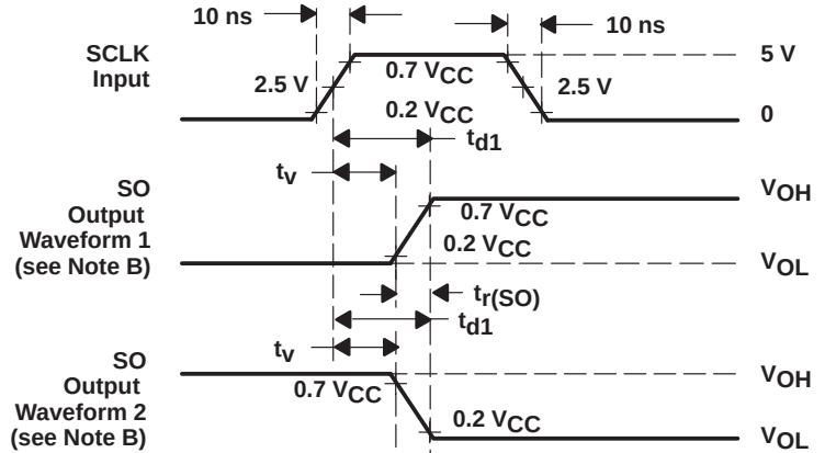
VOLTAGE WAVEFORMS
