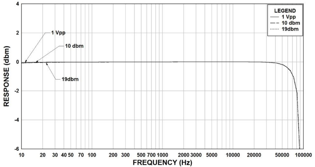
140UEX Rs=10K, RI=10K Frequency Response
