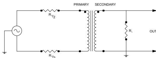
TYPICAL TEST CIRCUIT
