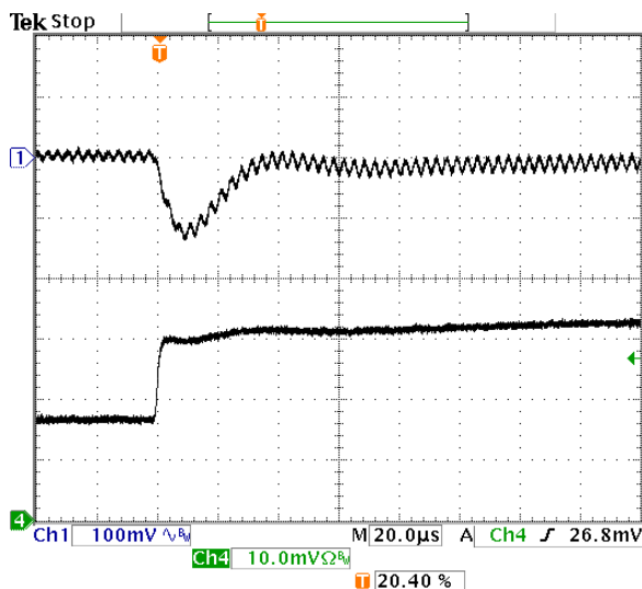
Fig-1.5V-6: Output voltage response for V_{out}=1.5V to positive load current step-change from 8A to 16A with slew rate of 5A/\mu s at V_{in}=5.0V . C_o=47\mu F \times 4 ceramic.
