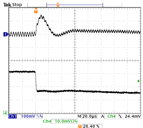
Fig-3.3V-7: Output voltage response for V_{out}=3.3V to negative load current step-change from 16A to 8A with slew rate of -5A/\mu s at V_{in}=5.0V . C_o=47\mu F \times 4 ceramic.
