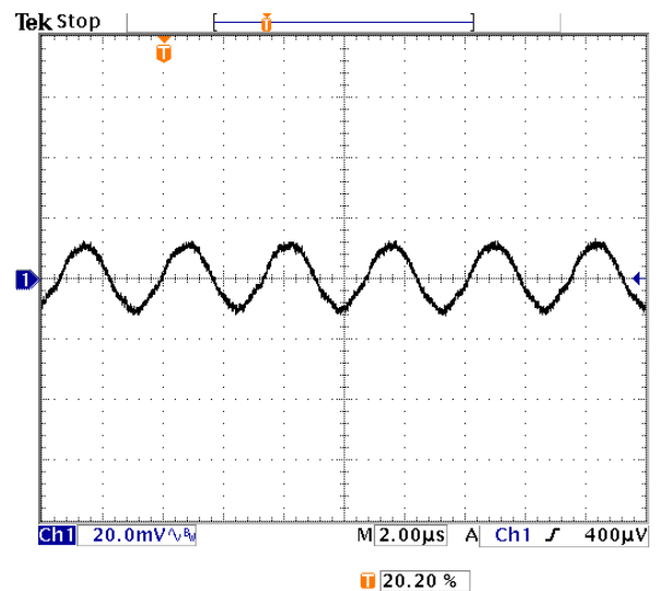
Fig-1.5V-5: Output voltage ripple (20mV/div.) for V_{out}=1.5V at full rated load current into a resistive load with external capacitance 47\mu F \times 4 ceramic + 1\mu F ceramic at V_{in}=5.0V .
