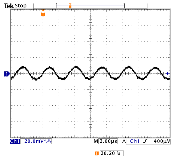
Fig-1.0V-5: Output voltage ripple (20mV/div.) for V_{out}=1.0V at full rated load current into a resistive load with external capacitance 47\mu F \times 4 ceramic + 1\mu F ceramic at V_{in}=5.0V .
