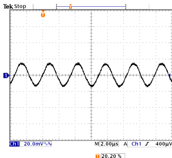
Fig-2.0V-5: Output voltage ripple (20mV/div.) for V_{out}=2.0V at full rated load current into a resistive load with external capacitance 47\mu F \times 4 ceramic + 1\mu F ceramic at V_{in}=5.0V .
