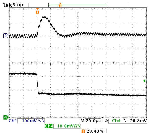
Fig-1.5V-7: Output voltage response for V_{out}=1.5V to positive load current step-change from 16A to 8A with slew rate of -5A/\mu s at V_{in}=5.0V . C_o=47\mu F \times 4 ceramic.
