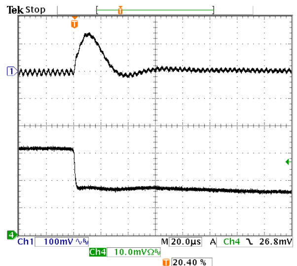
Fig-1.2V-7: Output voltage response for V_{out}=1.2V to positive load current step-change from 16A to 8A with slew rate of -5A/\mu s at V_{in}=5.0V . C_o=47\mu F \times 4 ceramic.
