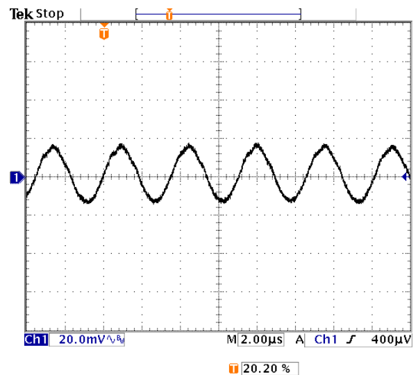
Fig-3.3V-5: Output voltage ripple (20mV/div.) for V_{out}=3.3V at full rated load current into a resistive load with external capacitance 47\mu F \times 4 ceramic + 1\mu F ceramic at V_{in}=5.0V .
