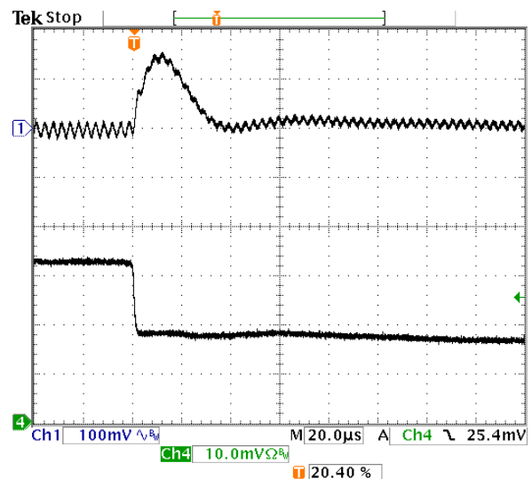
Fig-1.8V-7: Output voltage response for V_{out}=1.8V to positive load current step-change from 16A to 8A with slew rate of -5A/\mu s at V_{in}=5.0V . C_o=47\mu F \times 4 ceramic.
