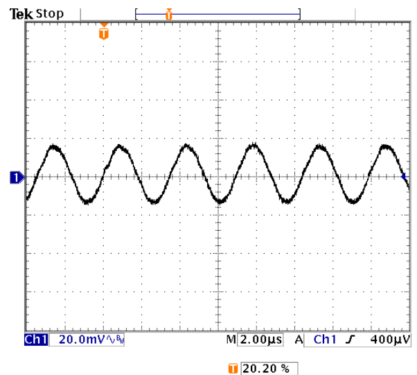
Fig-2.5V-5: Output voltage ripple (20mV/div.) for V_{out}=2.5V at full rated load current into a resistive load with external capacitance 47\mu F \times 4 ceramic + 1\mu F ceramic at V_{in}=5.0V .
