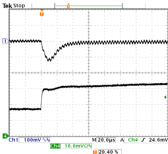
Fig-1.0V-6: Output voltage response for V_{out}=1.0V to positive load current step-change from 8A to 16A with slew rate of 5A/\mu s at V_{in}=5.0V . C_o=47\mu F \times 4 ceramic.
