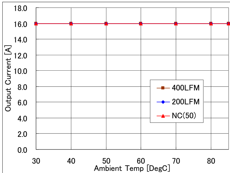
Fig-1.2V-1: Available load current vs. ambient temperature and airflow rates for Vout=1.2V with Vin=5.0V. Maximum component temperature \leq 120^{\circ}\text{C}
