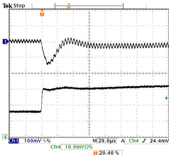
Fig-3.3V-6: Output voltage response for V_{out}=3.3V to positive load current step-change from 8A to 16A with slew rate of 5A/\mu s at V_{in}=5.0V . C_o=47\mu F \times 4 ceramic.
