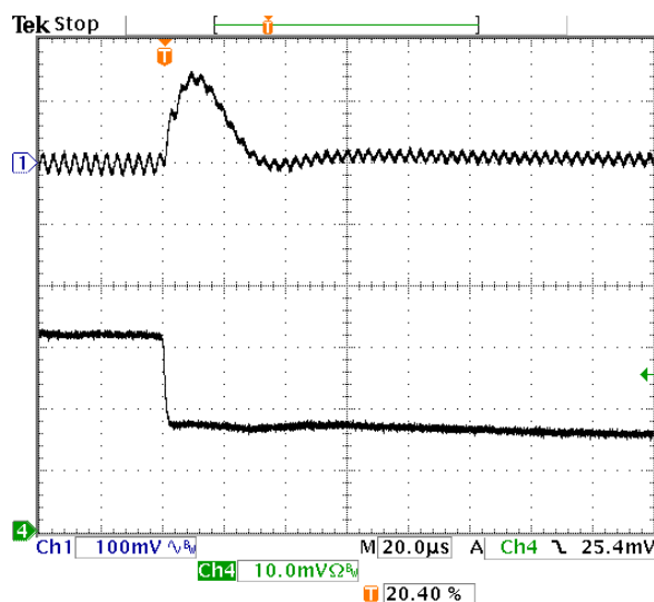
Fig-2.0V-7: Output voltage response for V_{out}=2.0V to positive load current step-change from 16A to 8A with slew rate of -5A/\mu s at V_{in}=5.0V . C_o=47\mu F \times 4 ceramic.
