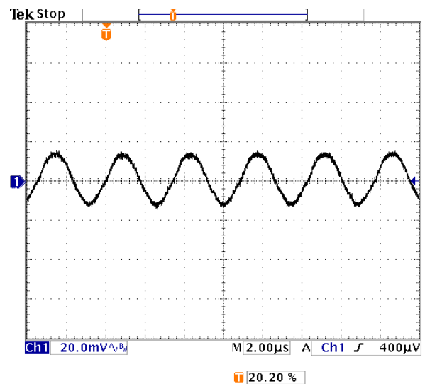
Fig-1.8V-5: Output voltage ripple (20mV/div.) for V_{out}=1.8V at full rated load current into a resistive load with external capacitance 47\mu F \times 4 ceramic + 1\mu F ceramic at V_{in}=5.0V .
