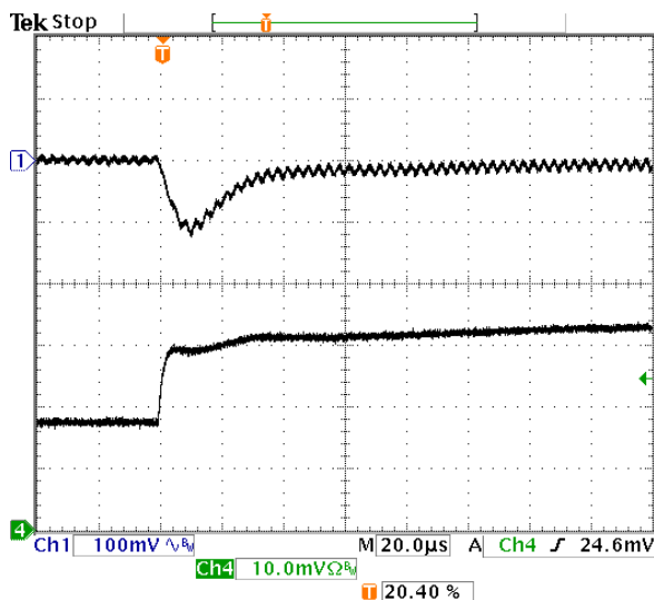
Fig-0.7525V-6: Output voltage response for V_{out}=0.7525V to positive load current step-change from 8A to 16A with slew rate of 5A/\mu s at V_{in}=5.0V . C_o=47\mu F \times 4 ceramic.
