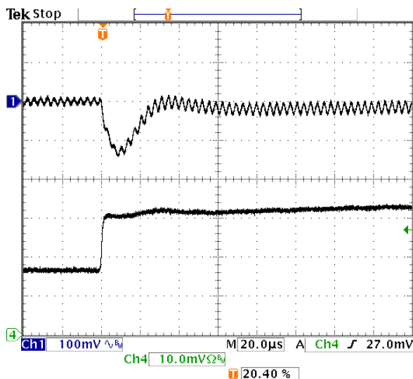
Fig-2.5V-6: Output voltage response for V_{out}=2.5V to positive load current step-change from 8A to 16A with slew rate of 5A/\mu s at V_{in}=5.0V . C_o=47\mu F \times 4 ceramic.
