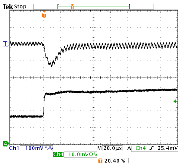
Fig-2.0V-6: Output voltage response for V_{out}=2.0V to positive load current step-change from 8A to 16A with slew rate of 5A/\mu s at V_{in}=5.0V . C_o=47\mu F \times 4 ceramic.
