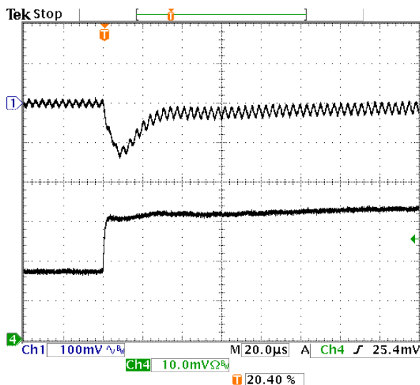
Fig-1.8V-6: Output voltage response for V_{out}=1.8V to positive load current step-change from 8A to 16A with slew rate of 5A/\mu s at V_{in}=5.0V . C_o=47\mu F \times 4 ceramic.
