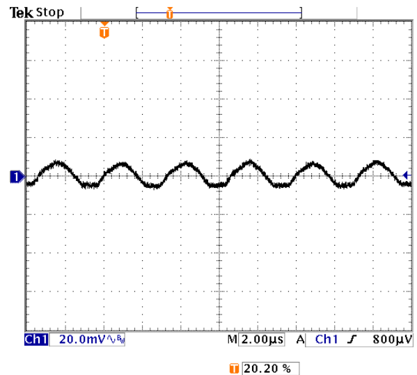
Fig-0.7525V-5: Output voltage ripple (20mV/div.) for V_{out}=0.7525V at full rated load current into a resistive load with external capacitance 47\mu F \times 4 ceramic + 1\mu F ceramic at V_{in}=5.0V .
