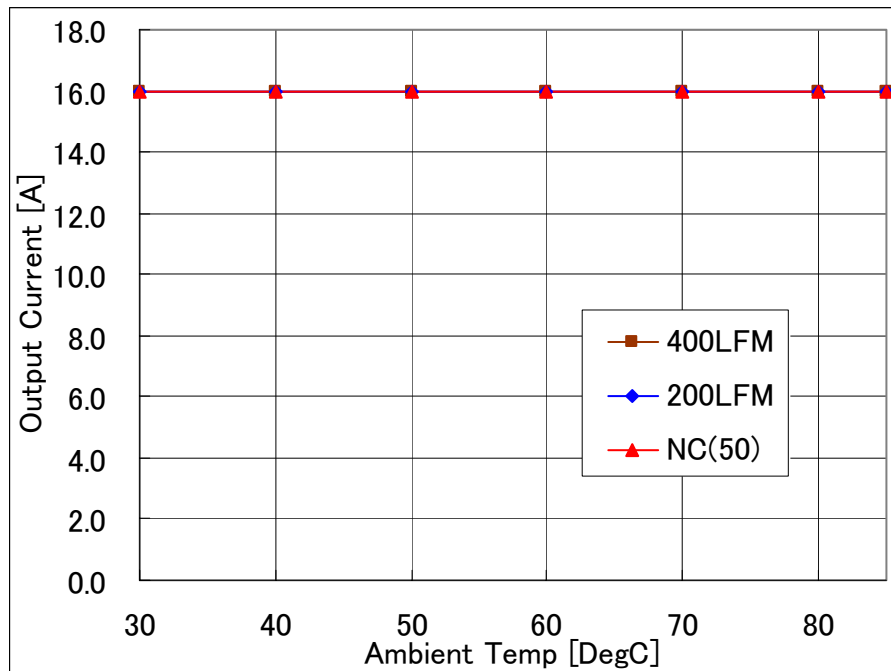
Fig-3.3V-1: Available load current vs. ambient temperature and airflow rates for Vout=3.3V with Vin=5.0V. Maximum component temperature \leq 120^{\circ}\text{C}
