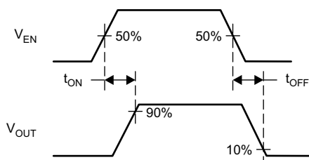
Figure 4. Enable Timing, Active High Enable
