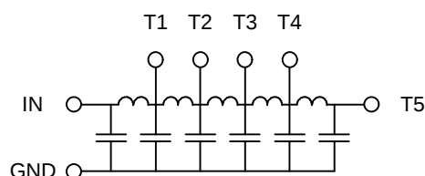
Functional Diagram
