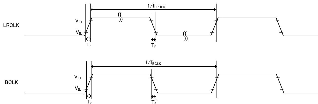
Figure 41. Clock timing
