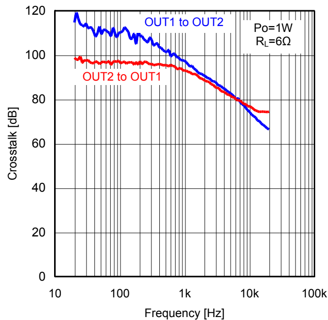
Figure 25. Crosstalk - Frequency
