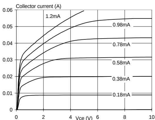
Fig.2. Typical transfer characteristics. I_C = f(V_{CE}) ; parameter I_B .
