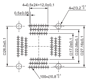
IC51-1004-809 (100 Pins)
