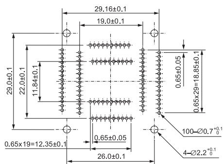
IC51-814-KS12033 (100 Pins)
