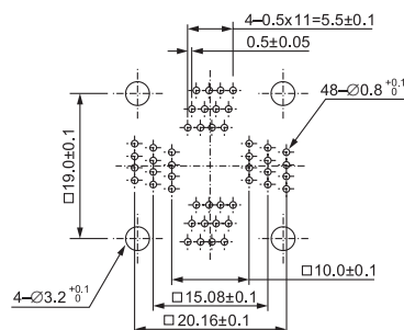
IC51-0484-806 (48 Pins)
