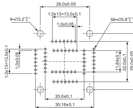
IC51-0564-790 (56 Pins)
