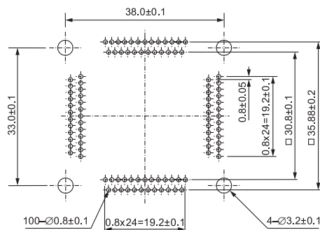
IC51-1124-1036-2 (112 Pins)
