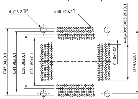
IC51-2564-1668 (256 Pins)
