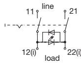
2-pole, unprotected
