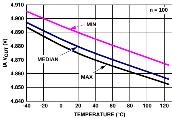
FIGURE 53. IA V_{OUT} HIGH vs TEMPERATURE, R_L = 1k , V_+ , V_- = \pm 2.5V
