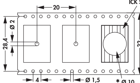
ICK SMD K 19
