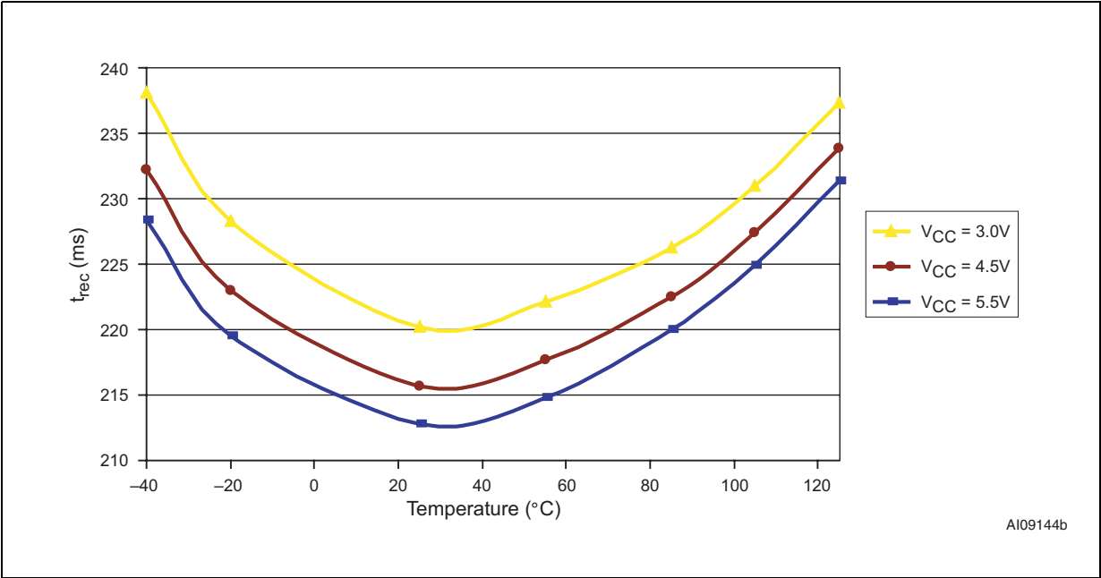
Figure 24. Power-up t_{\text{REC}} vs. temperature
