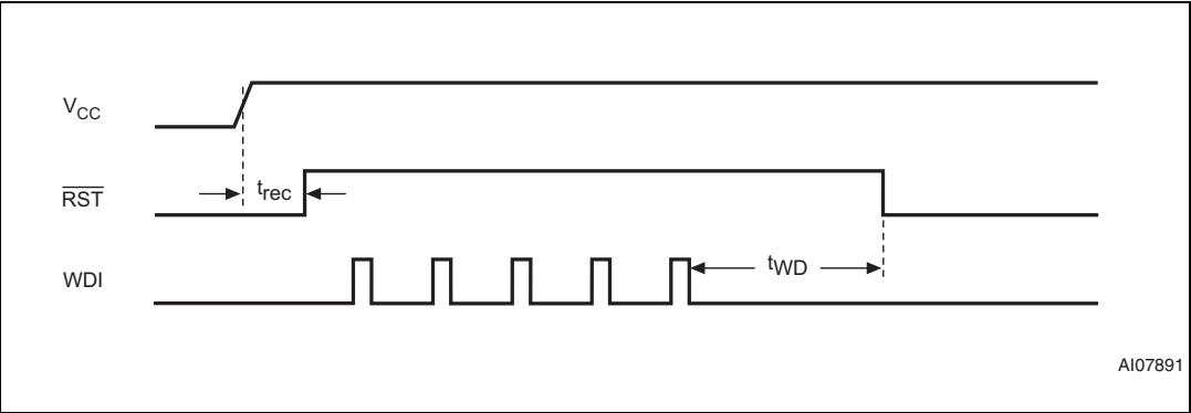
Figure 42. Watchdog timing
