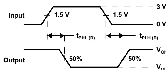
VOLTAGE WAVEFORMS
