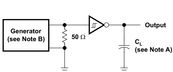
TEST CIRCUIT
