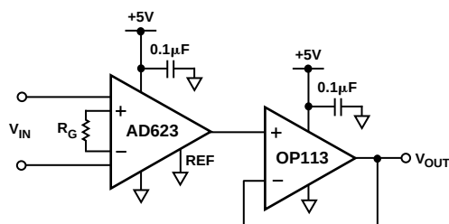
Figure 48. Output Buffering
