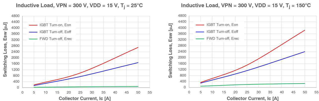
Figure 5. Switching Loss Characteristics
