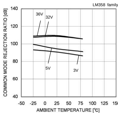
Fig. 23 Common Mode Rejection Ratio – Ambient Temperature
