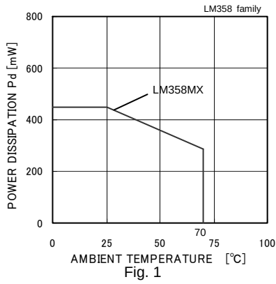
Fig. 1 Derating Curve
