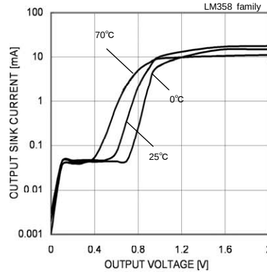
Fig. 8 Output Sink Current – Output Voltage ( V_{CC}=5[V] )
