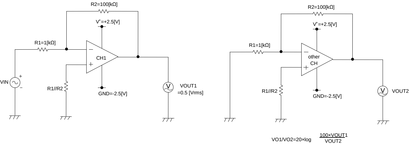
Fig.101 Measurement Circuit3
