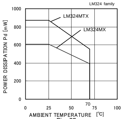
Derating Curve
