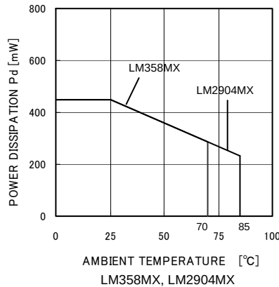
Power Dissipation
