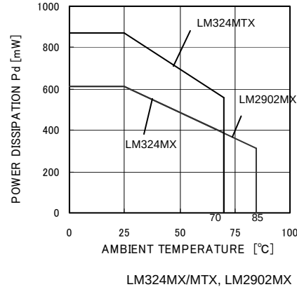
Power Dissipation
