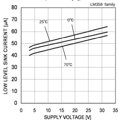
Fig. 10 Low Level Sink Current – Supply Voltage ( V_{OUT}=0.2[V] )
