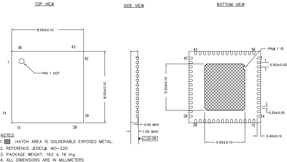
Figure 14. 56-pin QFN (8 x 8 x 1.0 mm) LT56B 4.5 x 5.2 E-Pad (Sawn) Package Outline, 001-53450
