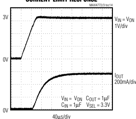
CURRENT-LIMIT RESPONSE
