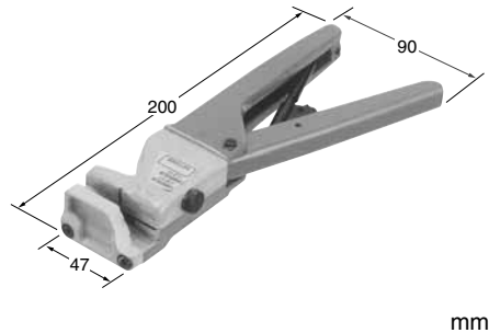
Pliers-type pressure welding tool for separate wires (with feed mechanism) AXY51000
