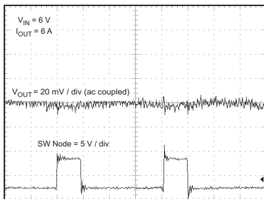
Figure 38. Output Ripple
