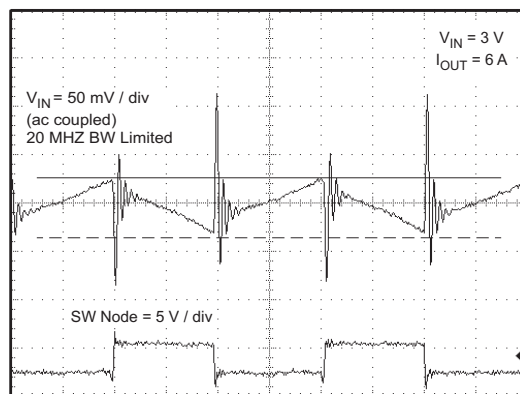
Figure 39. Input Ripple
