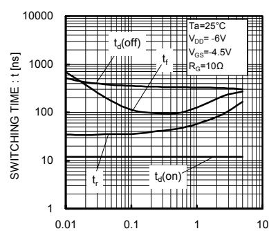
Fig.12 Switching Characteristics
