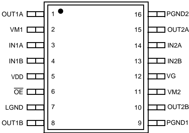
Figure 3. 17533 Pin Connections
