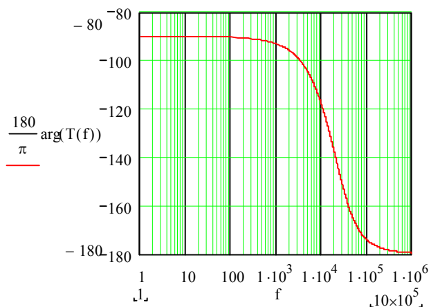
Figure 10. The loop transfer function Bode plot of the buck-boost example.
