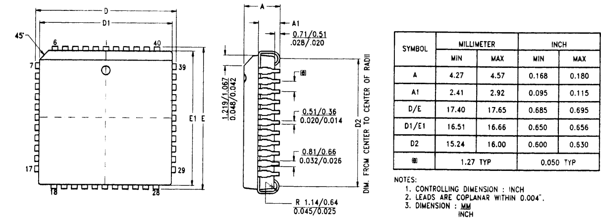
Figure 13. 44-Lead PLCC Package Diagram (for Prototype Only)
