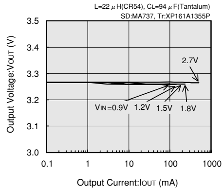
XC6368B102MR (180kHz, 3.3V)
