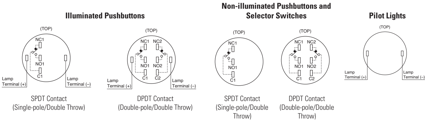
Terminal Arrangement (Top View)
