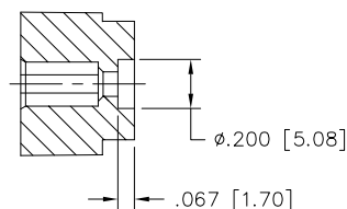
SECTION U-U
