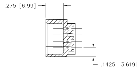
SECTION X-X
