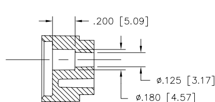
SECTION W-W
