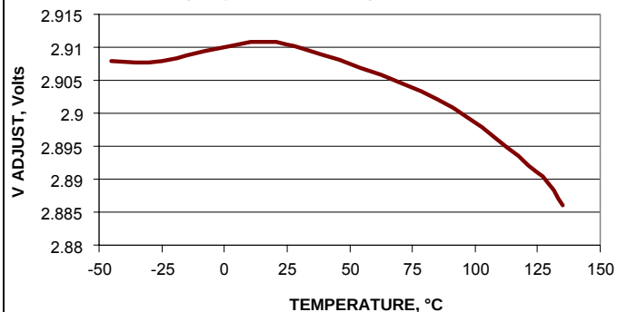
VOUT (Programmed to 2.9V) vs. TEMPERATURE
