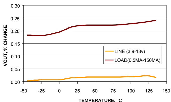
LINE and LOAD REGULATION
