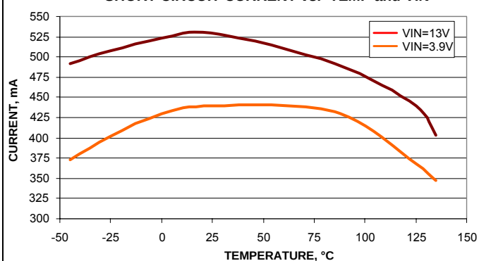
SHORT CIRCUIT CURRENT vs. TEMP and VIN
