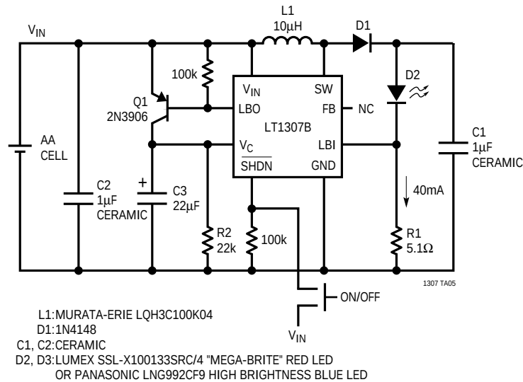
Single Cell Powered Constant Current LED Driver
