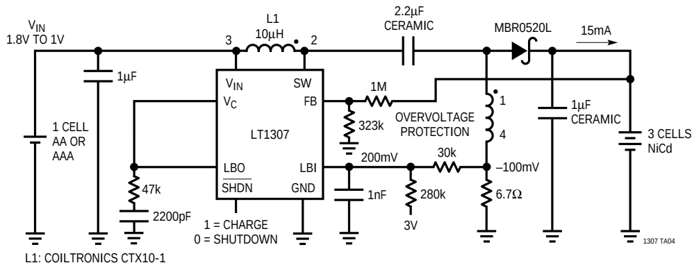
Constant Current NiCd Battery Charger with Overvoltage Protection for Acknowledge-Back Pagors
