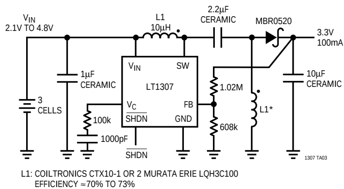
Step-Up/Step-Down Converter
