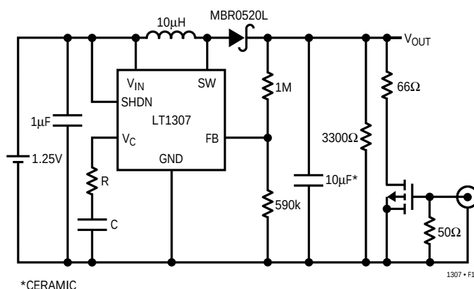
Figure 10. Boost Converter with Simulated Load
