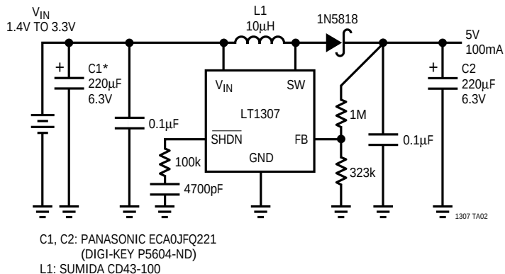
Low Cost 2-Cell to 5V
