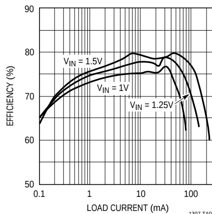
Single Cell to 3.3V Converter Efficiency
