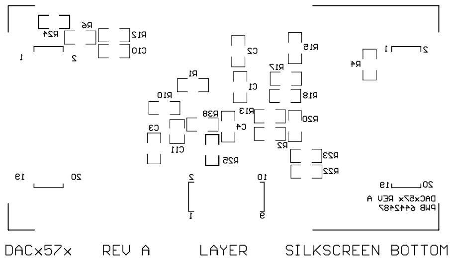
Figure 2-6. Bottom Silkscreen
