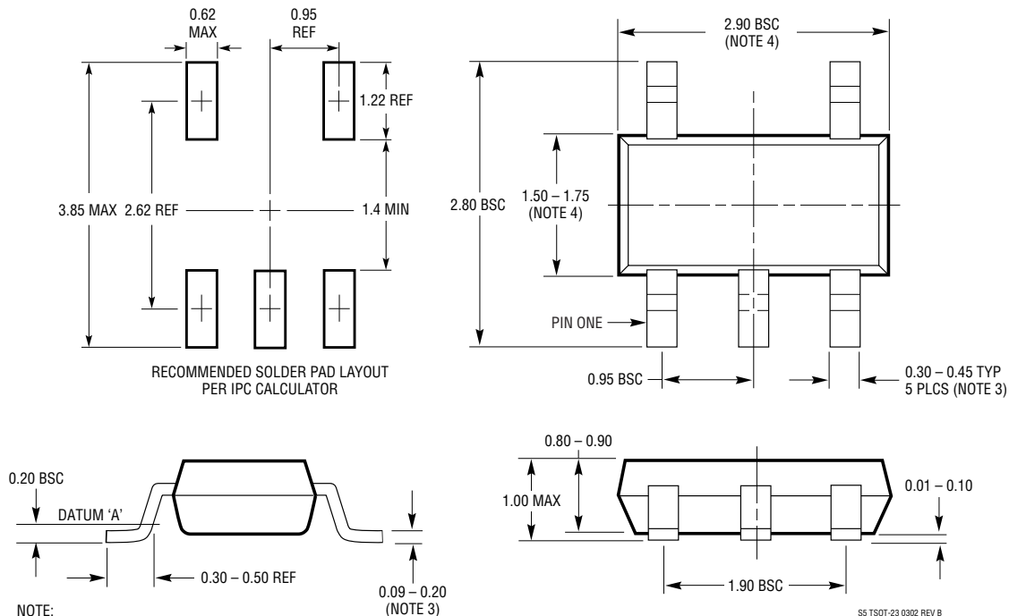
S5 Package 5-Lead Plastic TSOT-23 (Reference LTC DWG # 05-08-1717 Rev 0)
