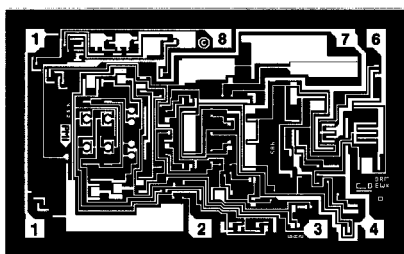
DIE SIZE 0.093 × 0.057 inch, 5301 sq. mils (2.36 × 1.45 mm, 3.42 sq. mm)
