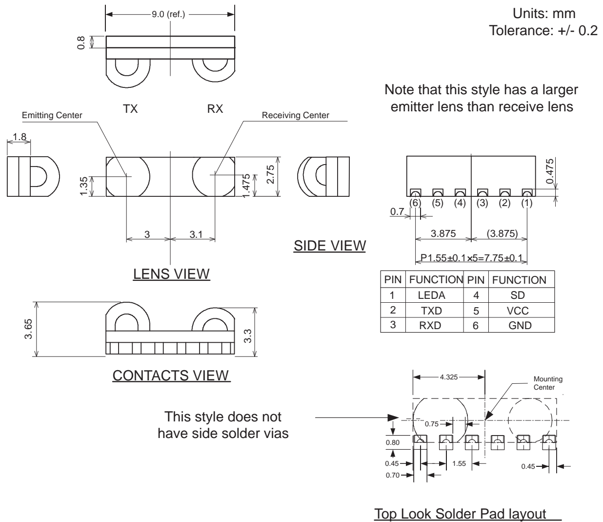
Figure 7. ZHX1820 Mechanical Drawing
