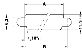
Housing cutout dimensions PSC 1,5/...M(-PE)
