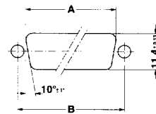
Panel cutout acc. to DIN 41 652-3 for walls up to 4.5 mm thick
