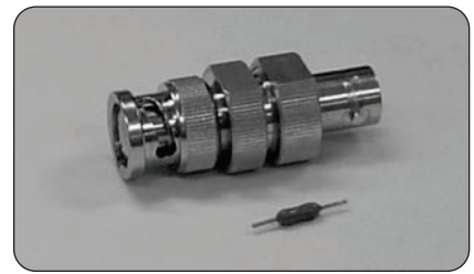
► BNC Fuse Adapter and 0.125 A Fuse.
