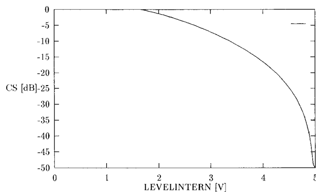
Figure 26. Internal stereoblend characteristics
