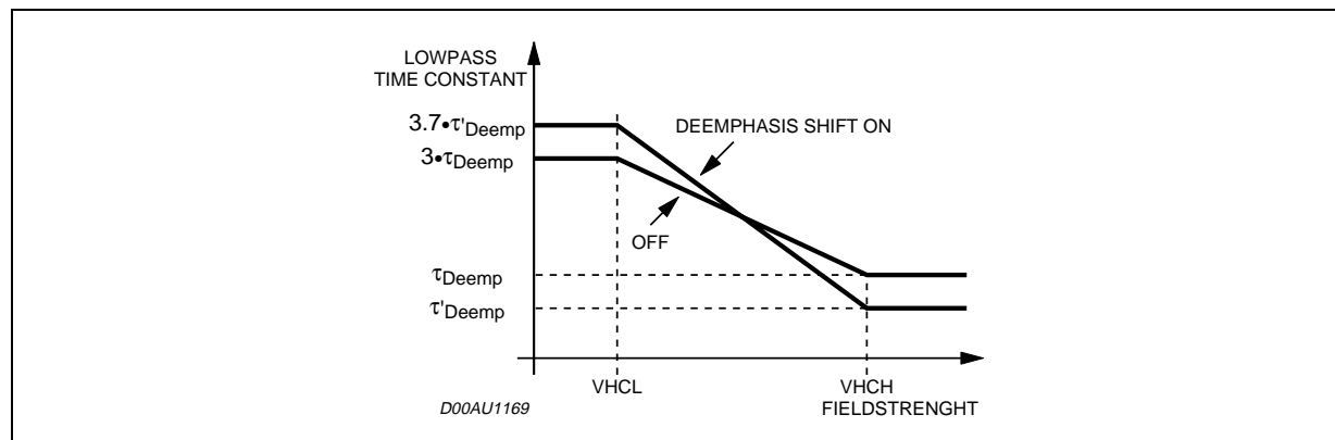
Figure 28. Highcut characteristics
