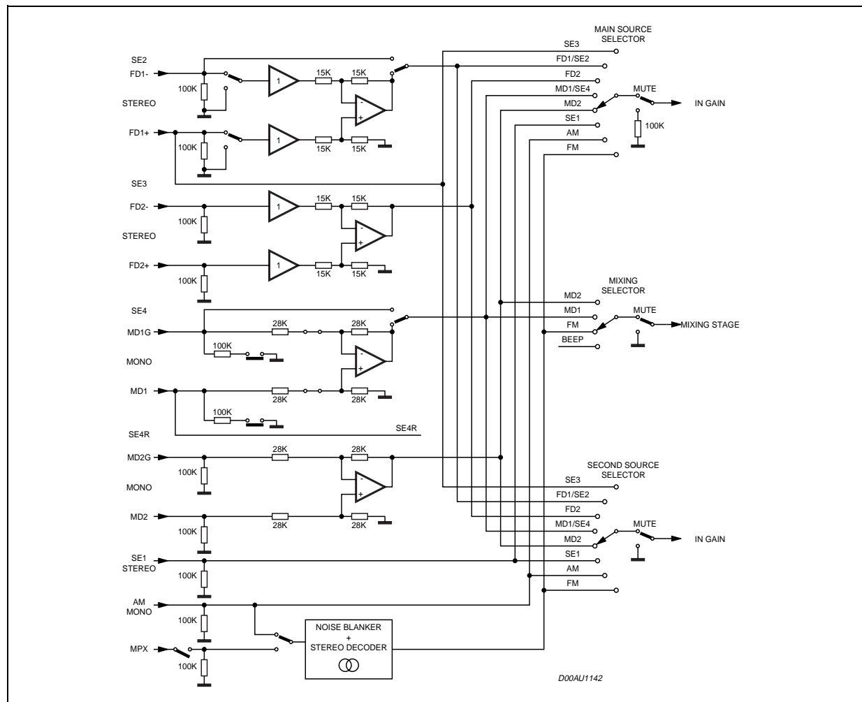
Figure 1. Input-stages
