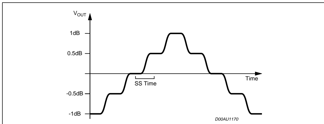
Figure 6. SoftStep-Timing
