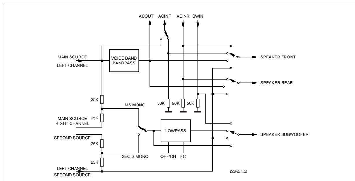
Figure 15. Output Selector
