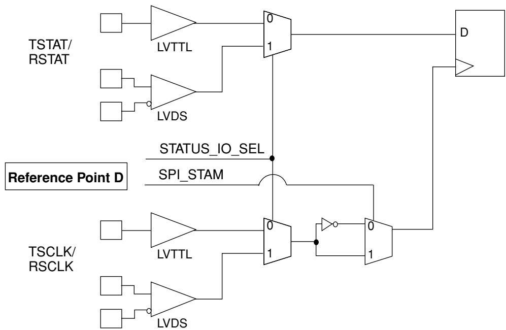
Figure 95. ORSPI4 Static Mode Status Signals Data Capture (Reference Point D)
