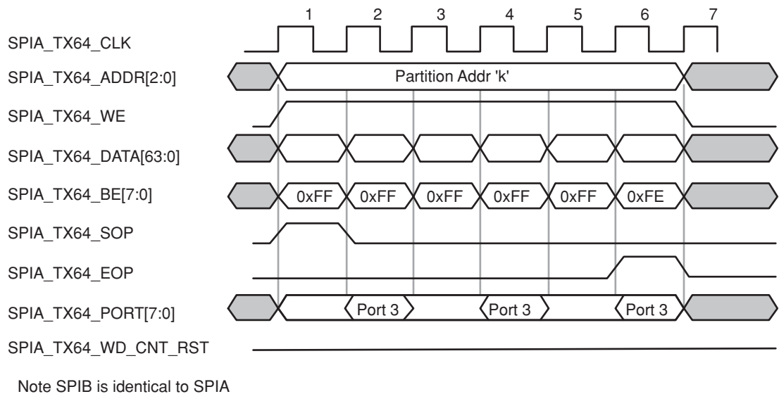
Figure 13. Basic 64-Bit Data Write Protocol to DPRAM
