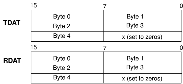
Figure 5. SPI4 Byte and Bit Ordering
