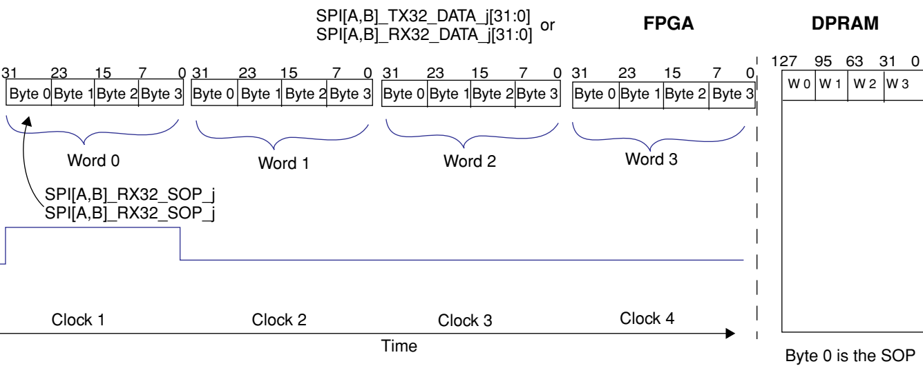
Figure 7. Byte and Bit Ordering in 32-Bit Operating Mode
