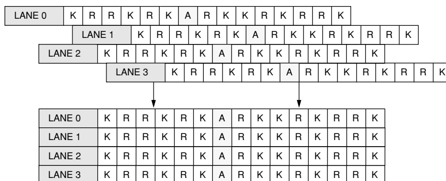
Figure 64. Deskew Lanes by Aligning /A/ Columns
